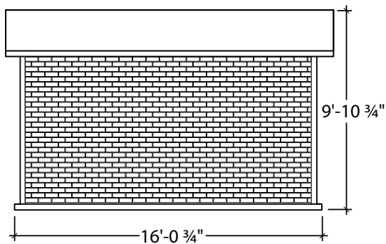
Right Side
